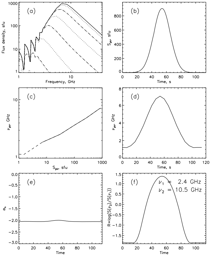
Figure 14 Spectral evolution of GS emission in the presence of high density plasma and continuous electron spectrum hardening, \delta = 4.0 - (t - t_{\max})/t_{\max} . The other parameters are the same as in Figure 13 except k = 10^3 and \phi = 45'' . Note the continuous increase of \nu_{pk} and R on the rise and decay phases. On panels (a) and (c) solid line is for the rising phase and dashed line for the decay phase.
