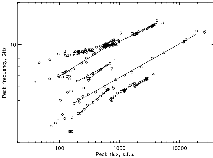
Figure 6 Peak frequency vs. peak flux density on the rise phase of seven events. The straight lines are the best linear fits (in logarithmic scale) near the peak of the bursts. The numbers indicate the events: 1–22 April 2001, 2–19 October 2001, 3–22 October 2001, 4–04 November 2001, 5–22 November 2001, 6–15 July 2002, 7–04 December 2002.
