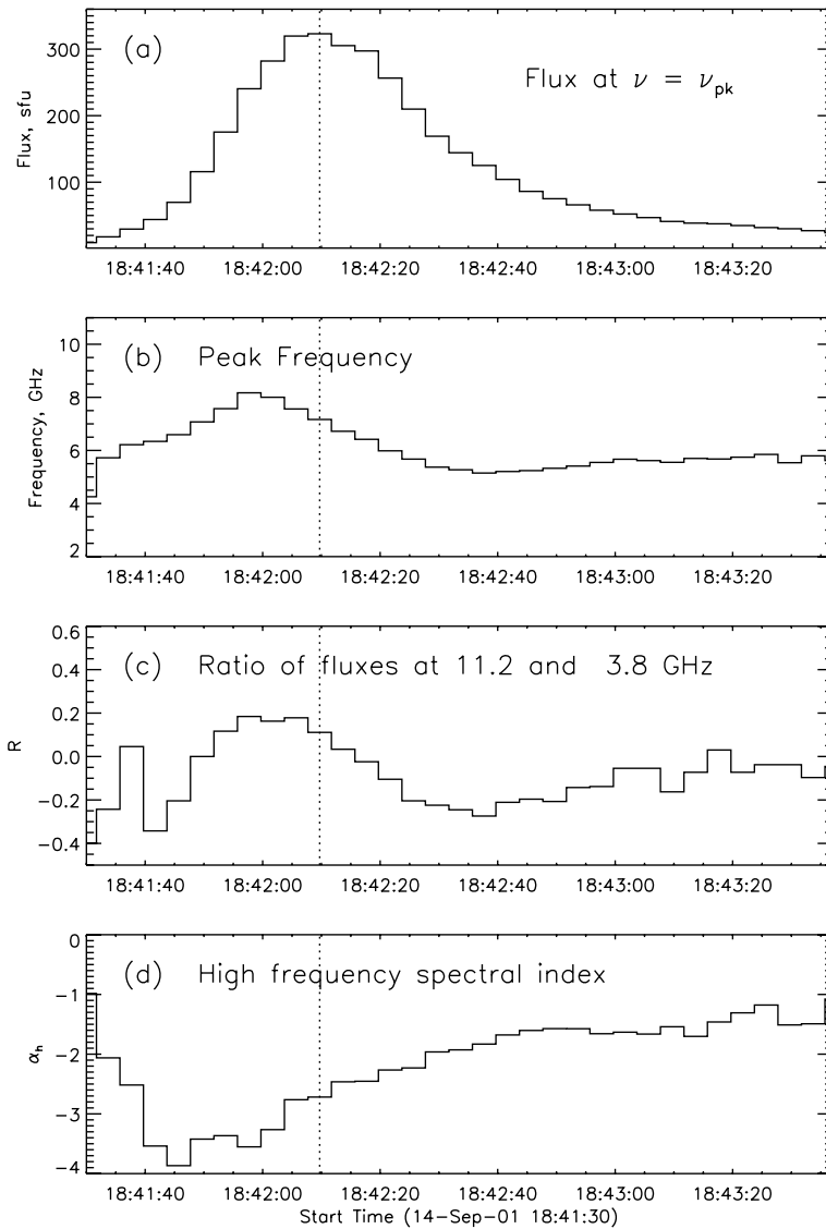
Figure 8 Time profiles as in Figure 3 for the bursts of 14 September 2001. This example shows a time delay between \nu_{pk} in (b) and S_{pk} in (a). Note also that on the decay \nu_{pk} first decreases and then slightly increases. The \alpha_h in (d) increases throughout the burst.
