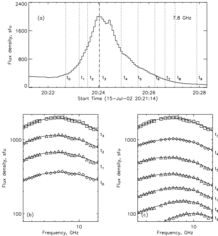
Figure 2 Spectral evolution as in Figure 1 for a secondary peak in the microwave burst of 15 July 2002. Note the remarkable stability of the peak frequency during the most of the burst, the equal rise and fall on both sides of the peak frequency (which yields a constant R ), and as well as its increase and steepening of the spectra at low frequencies on the late decay phase.
