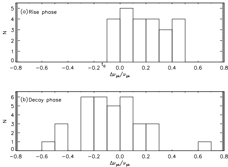
Figure 5 The distributions of shift in peak frequency, \Delta\nu_{pk}/\nu_{pk} , (a) on the rise and (b) decay phases. The corresponding flux density increase (decrease) is from (to) 25% of its maximum value. The total number of bursts used in the distributions is 24 in (a) and 34 in (b). Here \nu_{pk} is taken at the peak time of S_{pk}(t) .
