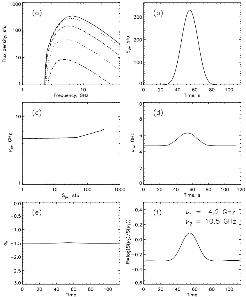
Figure 15 Spectral evolution of GS emission in the presence of high density plasma and electron spectral hardening, \delta = 4.0 - (t - t_{\max})/t_{\max} . The other parameters are the same as in Figure 13. The increase and decrease of \nu_{pk} and R in the main part of the emission peak is due to GS self-absorption. A new increase of the peak frequency and the flux ratio with time is clearly seen on the decay phase when the source becomes optically thin at low frequencies and the Razin suppression becomes dominant in defining the spectral peak.
