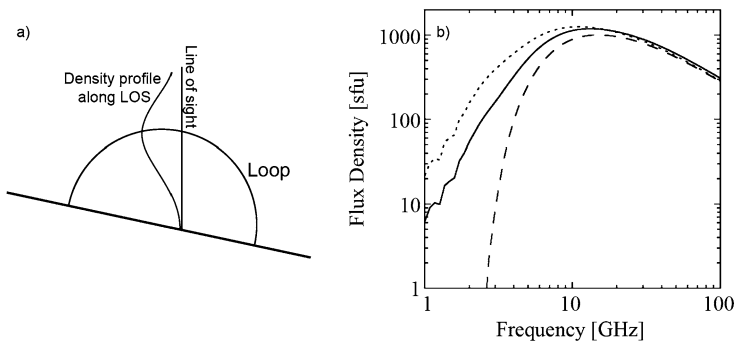
Figure 18 Influence of a plasma density inhomogeneity on the low frequency slope of the gyrosynchrotron spectrum. (a) Sketch of the model geometry used. The Gaussian curve shows the profile of both ambient and energetic electron density along the line of sight (see text for details). (b) Dashed line: The classical Razin suppressed spectrum as it would appear for a homogeneous source with the parameters on the loop axis. Solid line: The spectrum obtained along the line of sight in (a), due to the inhomogeneity in the model. Dotted line: The spectrum obtained with the same conditions as for the solid line spectrum, but with weighting to account for the radial dependence of area in a cylindrical geometry.
