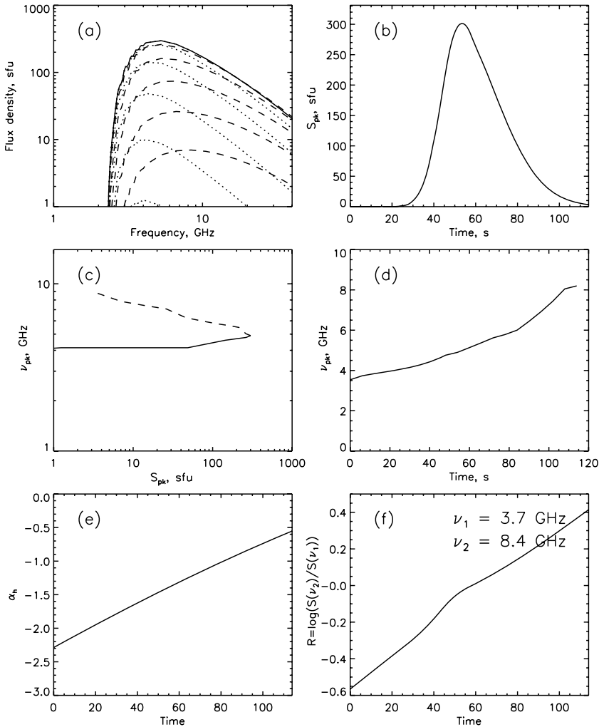
Figure 16 Spectral evolution of GS emission in the case of plasma density increase on the decay phase: n(t) = n_0[1 + 2(t - t_m)^2/t_m^2] , where n_0 = 5 \times 10^{10} \text{ cm}^{-3} , t_m = 200 \text{ s} . The other parameters are the same as in Figure 13, except \phi = 20'' . The increase of \nu_{pk} , R and \alpha_h on the late decay phase is completely due to the influence of high plasma density (Razin effect).
