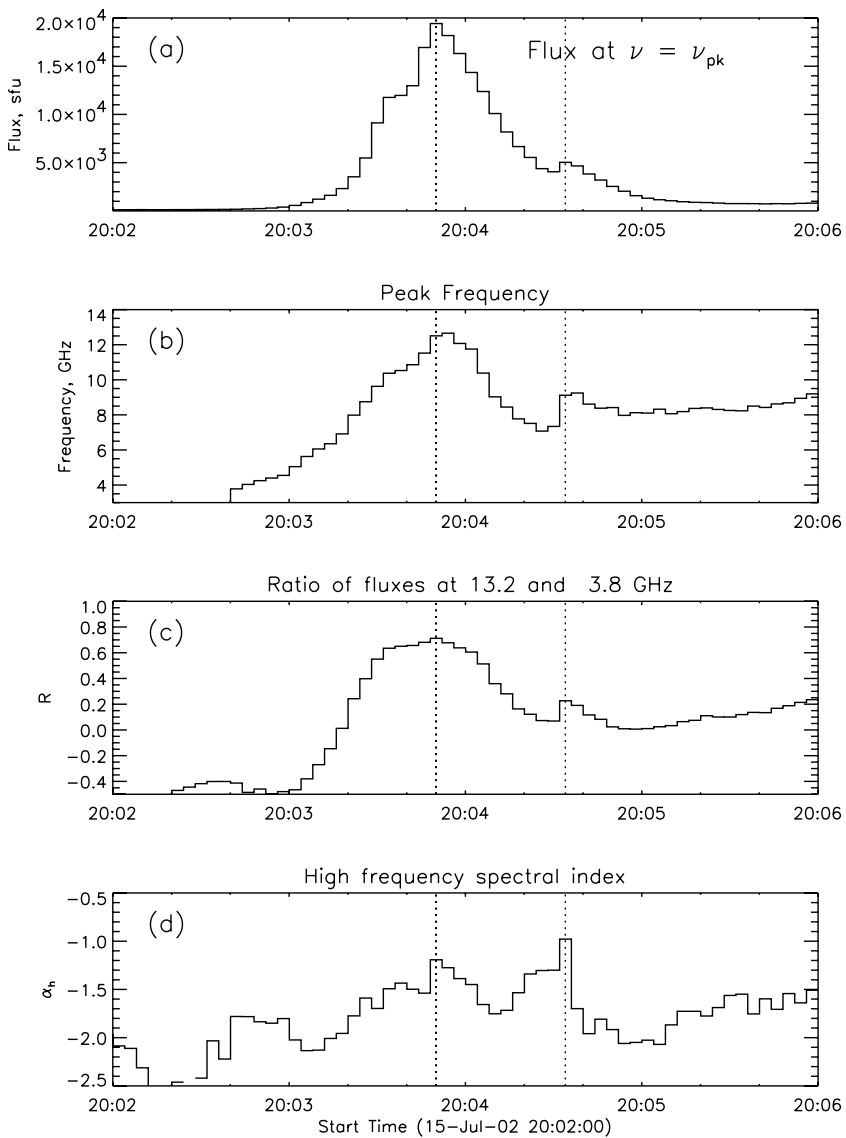
Figure 3 Time profiles of several key parameters of the spectral evolution of the burst shown in Figure 1: (a) Flux density, (b) peak frequency, (c) ratio R of fluxes at two frequencies, one (13.2 GHz) on the high-frequency side and one (3.8 GHz) on the low-frequency side of \nu_{\text{pk}} , and (d) the high frequency spectral index, \alpha_h . A strong correlation is seen among the top three panels, both on the rise phase and initial part of the decay phase. The dotted vertical lines in each panel mark the peak times in panel (a).
