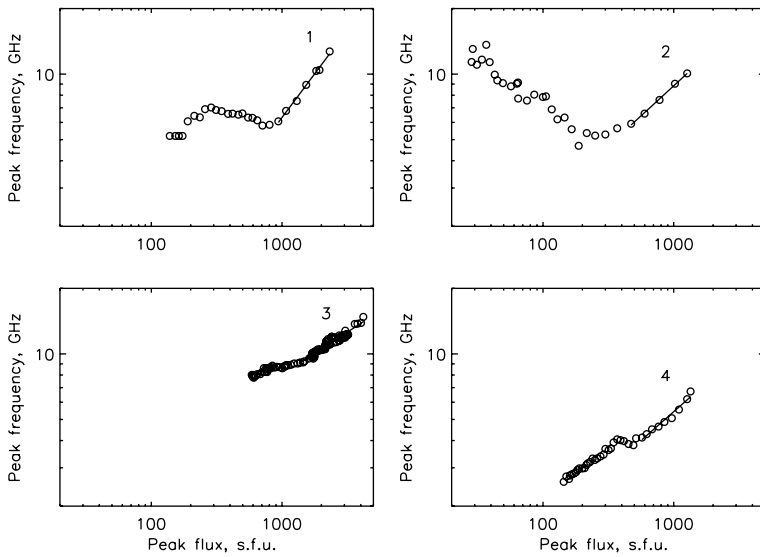
Figure 13 Spectral evolution of GS emission in the presence of high density plasma: n_0 = 5 \times 10^{10} \text{ cm}^{-3} . The other parameters are same as in Figure 12. The low frequency turnover is determined by two effects: (1) by the Razin suppression on the initial rising phase and late decay phase, and (2) by the self-absorption near the maximum of the simulated burst. Note the high initial value and small range of the peak frequency and R variations.
